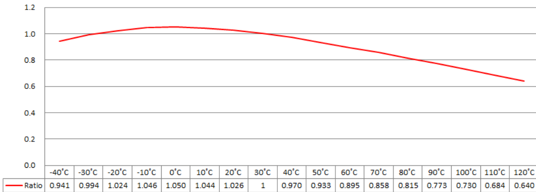
WCS1800 Sensitivity standardization of 30°C (3.3V) V.S Temperature
