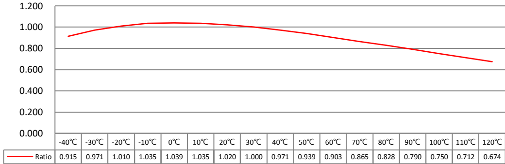
WCS2320 Sensitivity standardization of 30°C (3.3V) V.S Temperature
